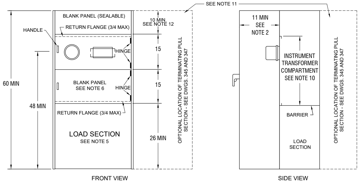
APS DWG. 1101.1 ALL DIMENSIONS SHOWN ARE IN INCHES
