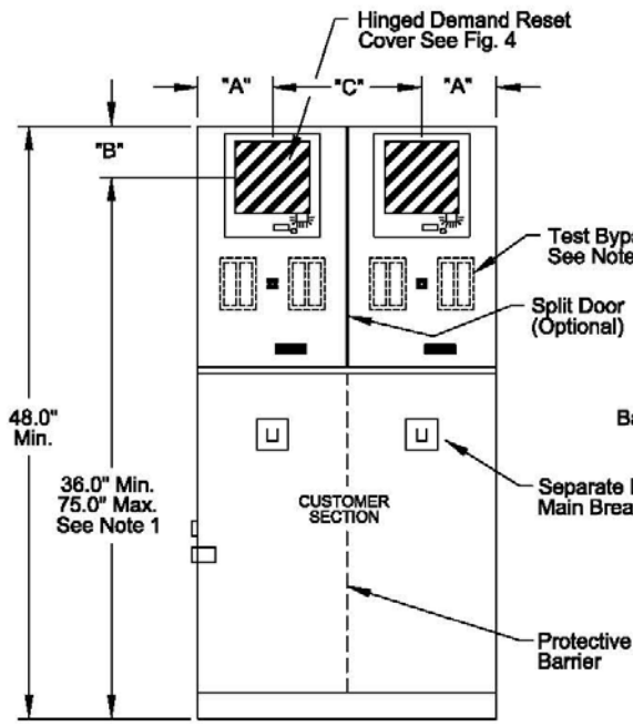
Fig. 1 FRONT VIEW
