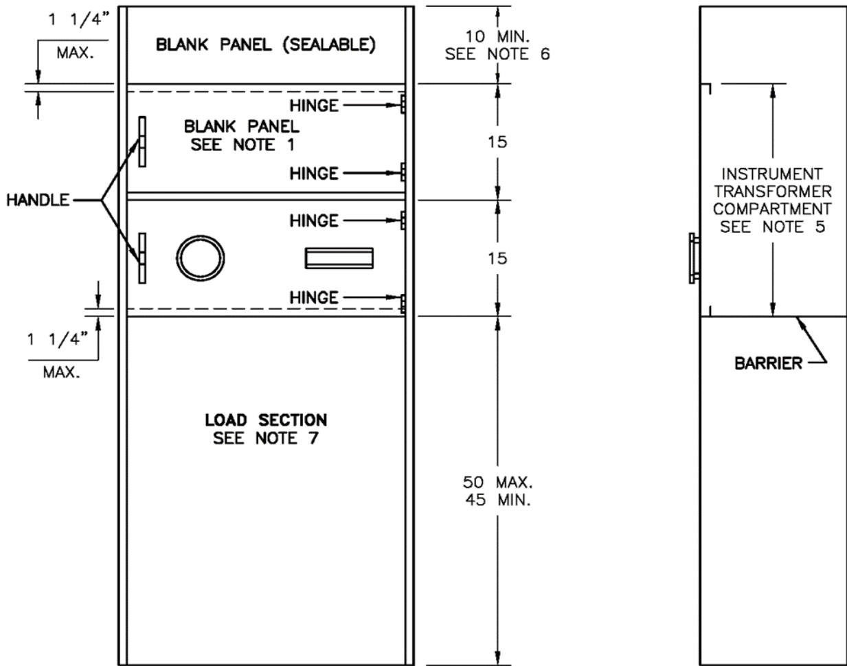
FRONT VIEW
