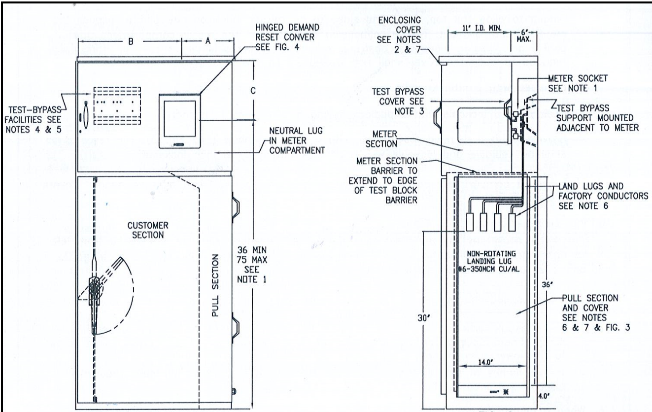
FIG. 1 FRONT VIEW
